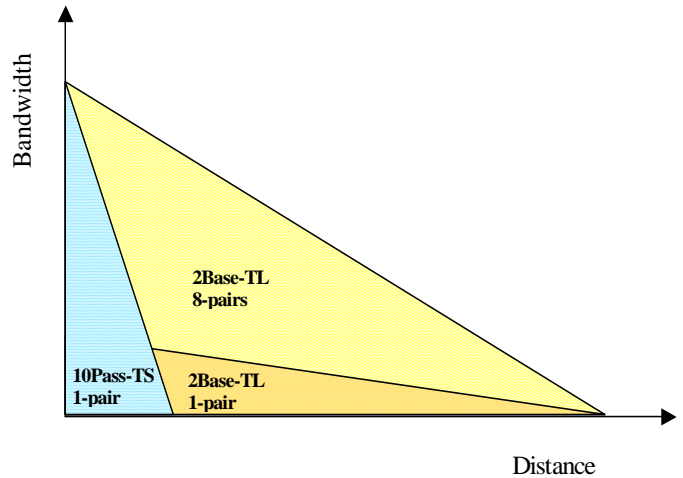
Figure 11: Short and Long Reach Options for EFMC
