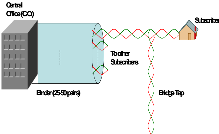
Figure 7: PSTN Loop plant
