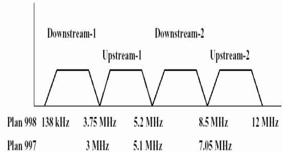
Figure 12: EFMC Short reach PHY Details
