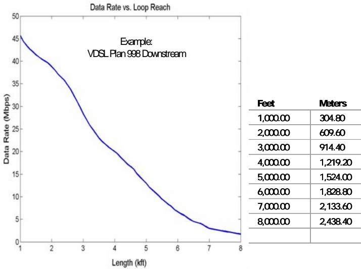
Figure 10: Sample Data Rate versus Loop Reach (Downstream VDSL)
