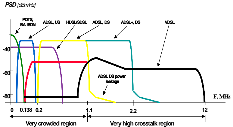
Figure 8: Band Plan Definitions
