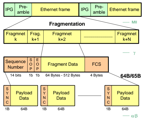
Figure 6: EFM Fragmentation and Framing
