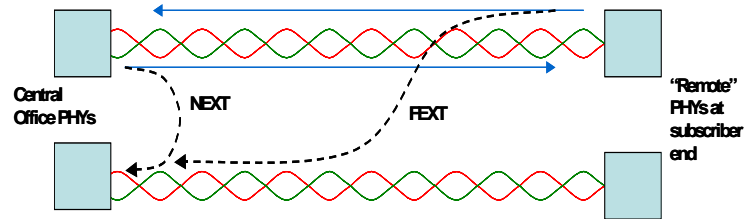
Figure 9: Far End and Near End Crosstalk
